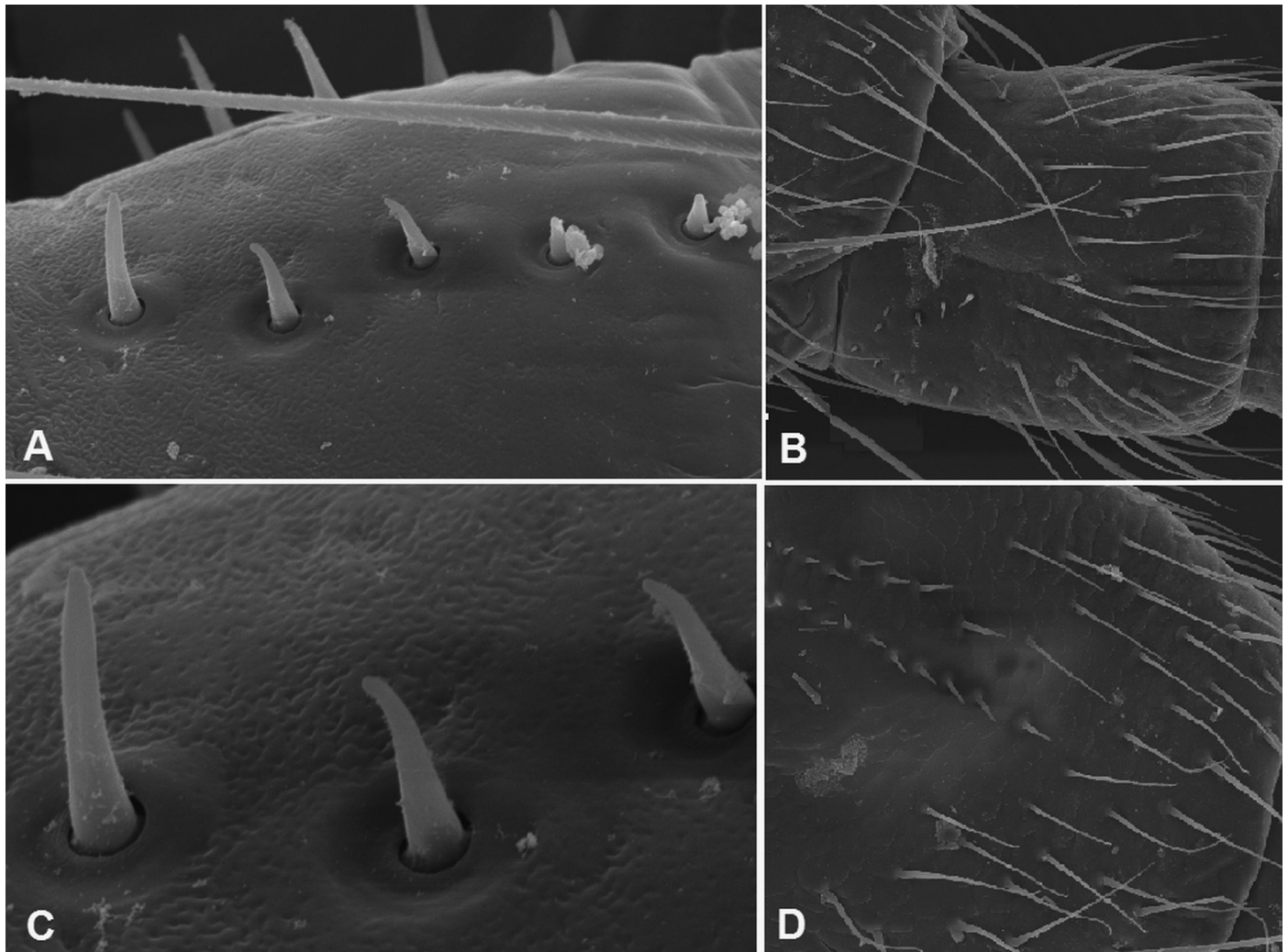
Fig. 2. Böhm sensilla ( Bs ) (SEM, \times 1.1k and \times 2K) (A, B) on the S. abbreviatus pedicel ( \times 500) (C) and scape ( \times 650) (D).
