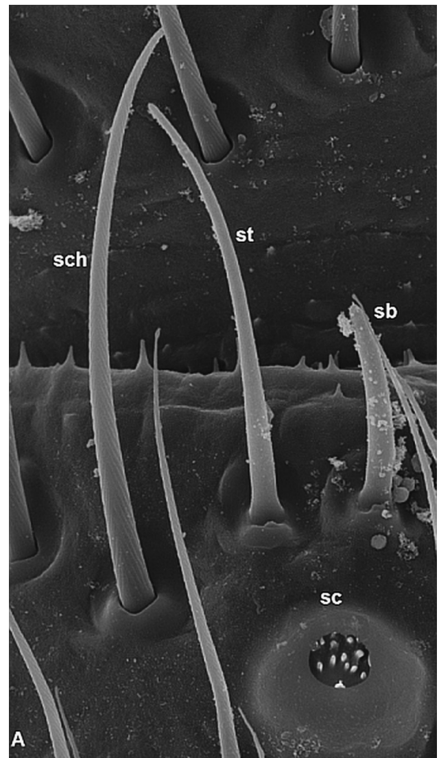
Fig. 6. Short s. basioconica ( \times 22k and 15k ) (sb) (A), arranged in transverse row on the apical part of antennal segment of N. hexadactyla ( \times 900 ) (B).
