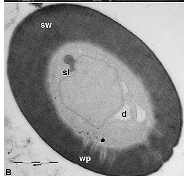
Fig. 7. Sensillum trichodium (st) located at the distal part of flagellomere together with s. chaeticum (sch), s. basioconicum (sb) and s. coeloconicum (sc) ( \times 9k ) (A); cross-section of s. trichodium (B) showing presence of the sensillum lumen (sl) with dendrites (d) and thick wall (sw) with pores (wp) (C).
